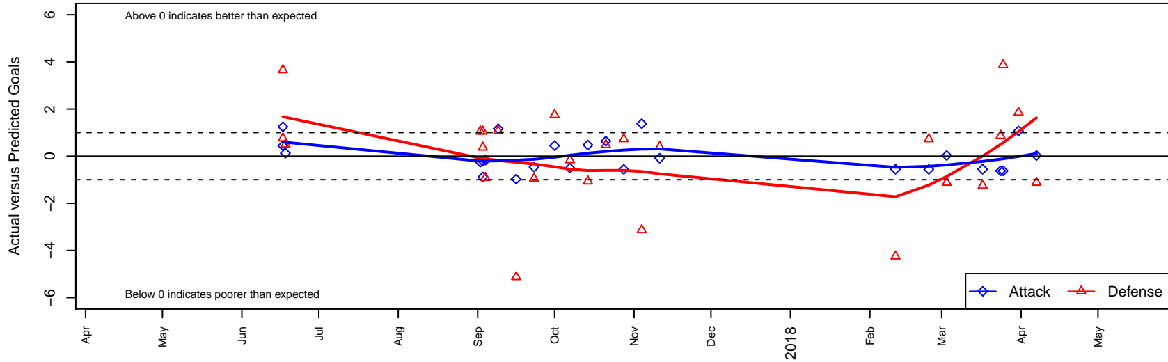
NC Alliance Rebels B05 Dots are actual minus expected GF (blue circles) and GA (red triangles). Blue line is smoothed change in attack strength. Red is smoothed change in defense strength.
